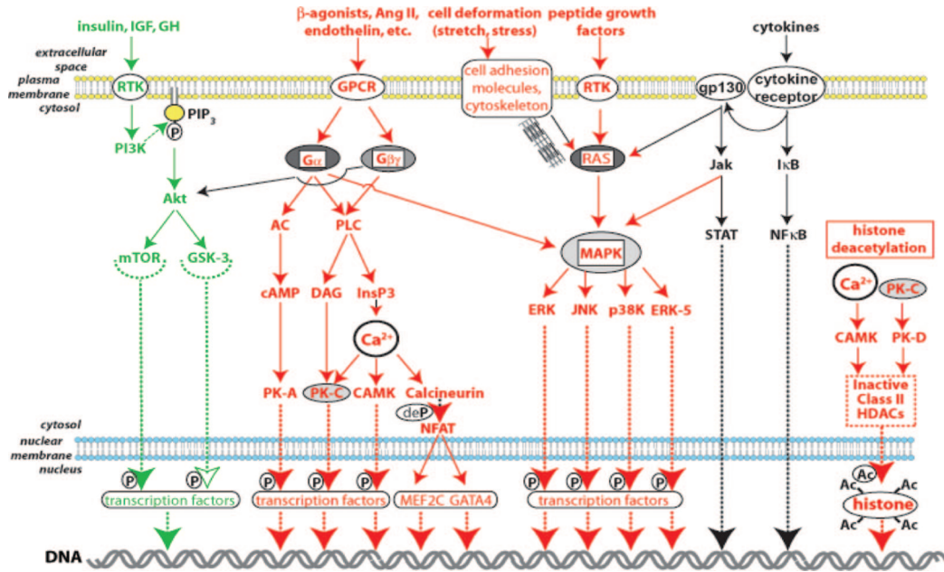
Figure 5. Proliferative signaling pathways that mediate cardiac hypertrophy. The PI3K/PIP 3 /Akt pathway is activated when insulin, insulin growth factor (IGF), and growth hormone (GH) bind to receptor tyrosine kinases (RTK); the cascade begins with phosphorylation of phosphatidylinositol tris phosphate (PIP 3 ) by phosphoinositide 3'-OH kinases (PI3K) that activates Akt, a protein kinase that phosphorylates mammalian target of rapamycin (mTOR) and inhibits glycogen synthetase kinase 3 (GSK-3). Neurohumoral mediator binding to G-protein-coupled receptors (GPCR) activates G α and G βγ . G αs activates adenylyl cyclase (AC) to form cyclic adenosine monophosphate, which stimulates protein kinase A (PK-A). G αq and G βγ activate phospholipase C (PLC) to form diacylglycerol (DAG) and inositol tris phosphate (InsP 3 ). DAG stimulates protein kinase C (PK-C). Calcium released by InsP 3 activates protein kinase C and calcium/calmodulin kinase (CAMK). Calcium also activates calcineurin, a protein phosphatase that dephosphorylates nuclear factor of activated T cell (NFAT) so as to activate the transcription factors MEF2C and GATA4. Peptide growth factor binding to RTKs and cytoskeletal signaling pathways activate Ras, a monomeric G-protein that stimulates mitogen-activated protein kinase (MAPK) pathways; the latter include extracellular receptor-mediated kinases (ERK), c-Jun kinase (JNK), and p38 kinase (p38K). Activated cytokine receptors release an inhibitory effect of I \kappa B on nuclear factor- \kappa B (NF \kappa B) and activate gp130-mediated signaling pathways that stimulate janus kinase (Jak) to activate signal transducer and activator of transcription (STAT) and MAP kinases. Calcium and protein kinase C can inactivate class II histone deacetylases (HDACs), which increase histone acetylation (Ac) that reduces an inhibitory epigenetic effect on DNA transcription. Pathways in red mediate mainly maladaptive hypertrophy; those in green, mainly adaptive hypertrophy. Cytokine-activated pathways (black) can activate both adaptive and maladaptive growth. Thin solid arrows indicate signaling pathways; dotted arrows with solid arrowheads, phosphorylations (P); and those with open arrows, dephosphorylations (deP). Modified from Katz. 40
