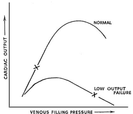
Figure 3. Diagram illustrating the failing heart operating on the descending limb of the Starling curve. Adapted from McMichael. 20
