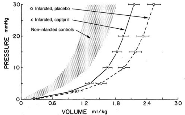
Figure 4. Effect of the ACE inhibitor captopril on left ventricular diastolic pressure-volume relationships after myocardial infarction. Diastolic volumes and pressures are shown for noninfarcted control rats (shaded area, mean \pm 2 SD), infarcted hearts of untreated rats (o), and infarcted hearts of rats treated with captopril (x). Data derived from Pfeffer et al. 62
